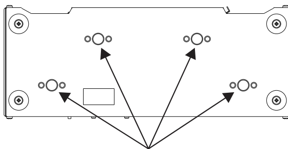
Figure 3-3: Camlock Sockets
