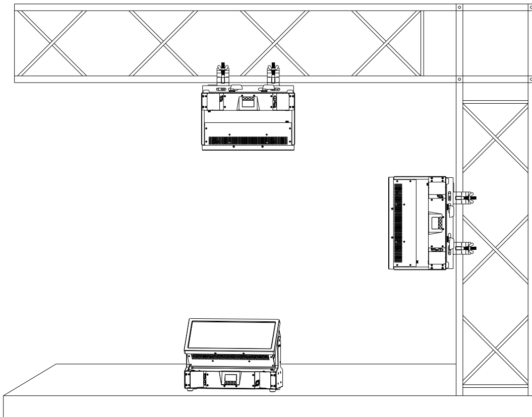
Figure 3-1: Mounting Options (safety cable not shown)
